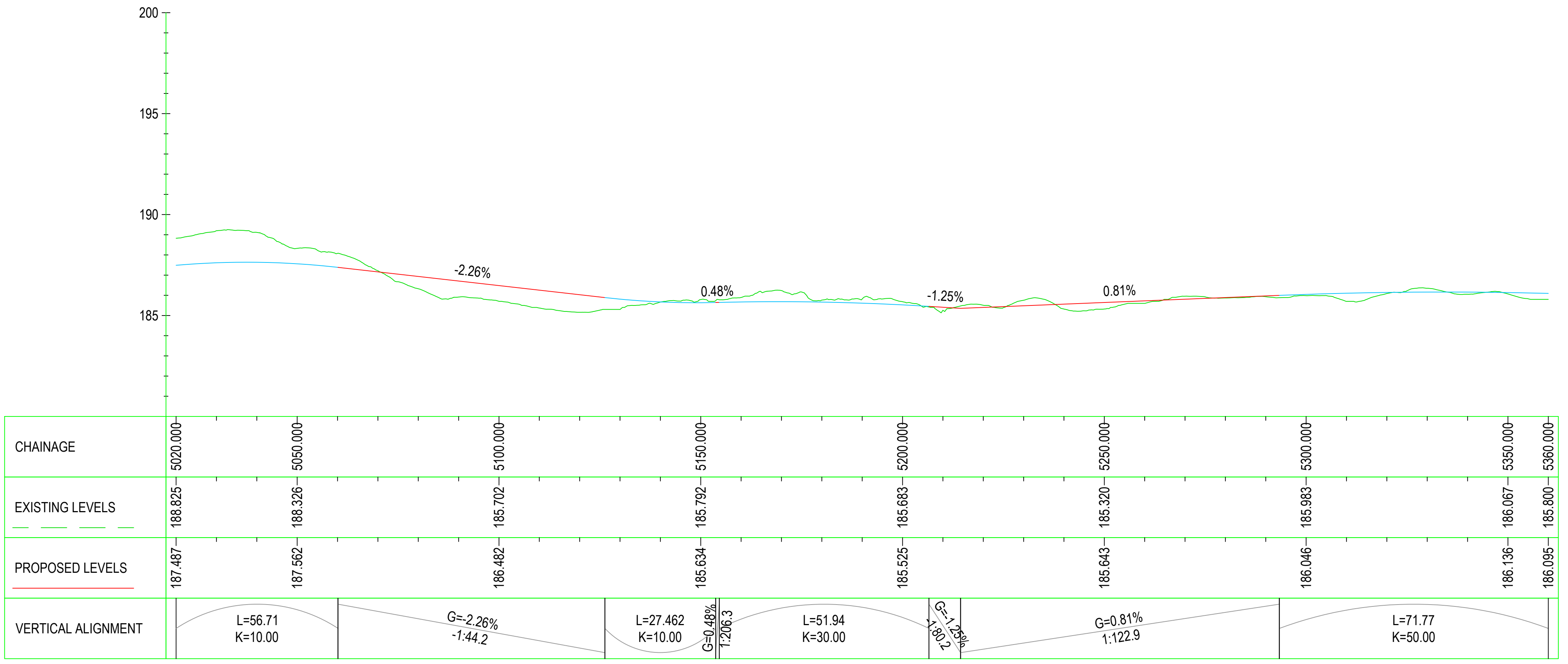
BLESSINGTON ALIGNMENT LONGSECTION SCALE: H 1:1000, V 1:200
